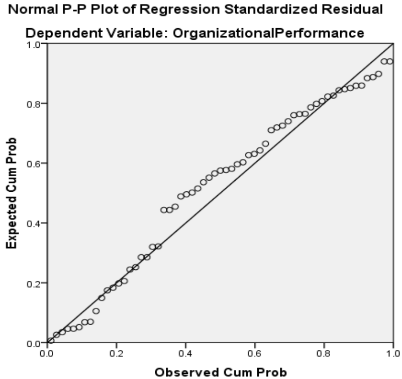
Figure 4.4: Normal PP Plot
