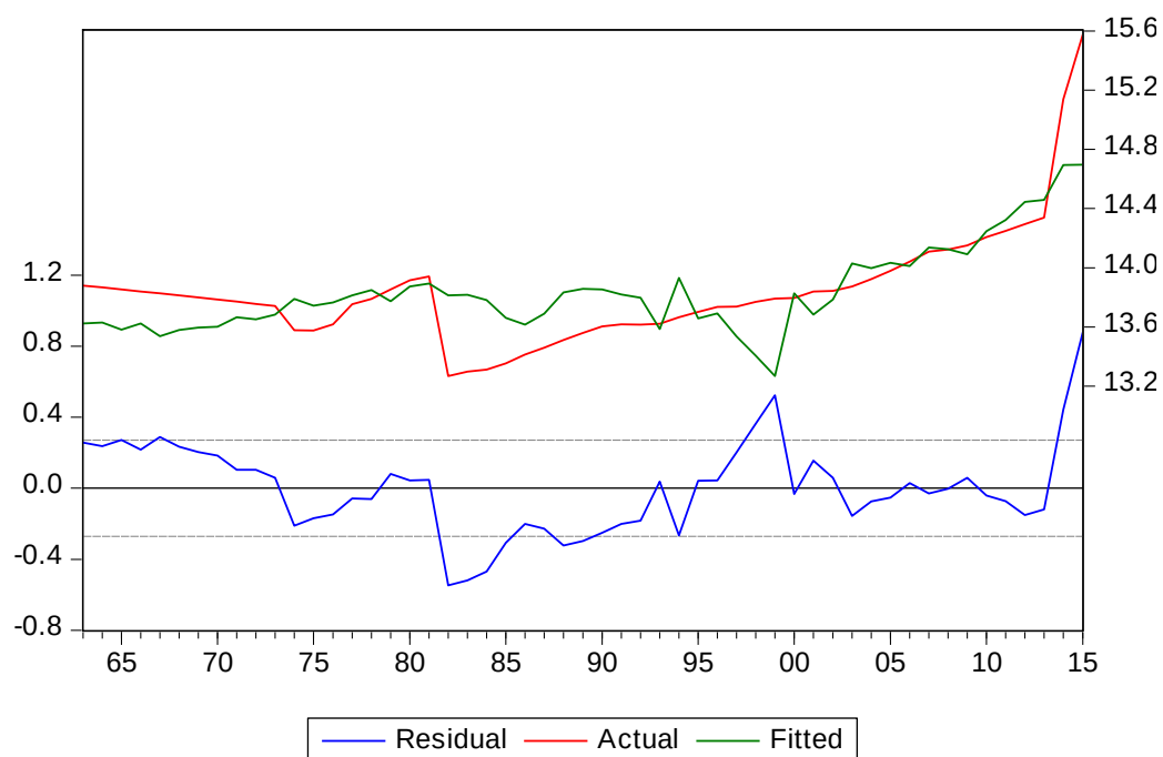
Figure 4.5 Residual Plot
