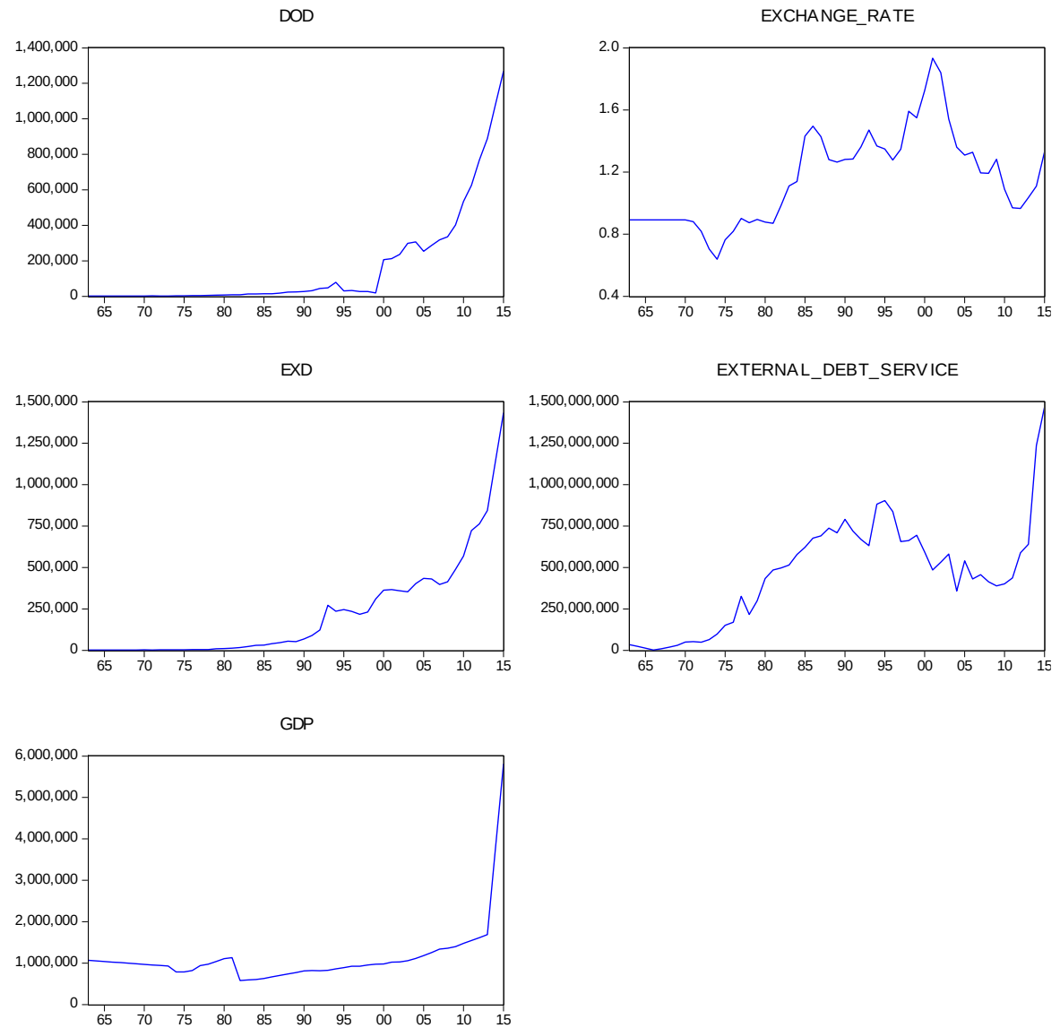
Figure 4.1 Trend analysis
