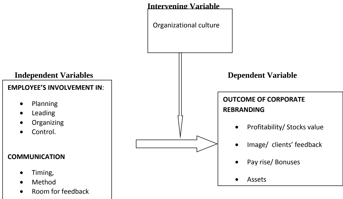
Figure 1: Conceptual Framework
